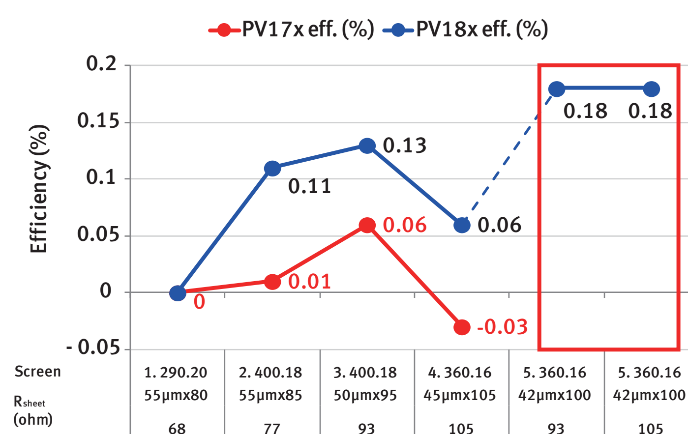
Over 0.1% efficiency improvement achieved by DuPont™ Solamet® PV18x due to its superior fine line capability
