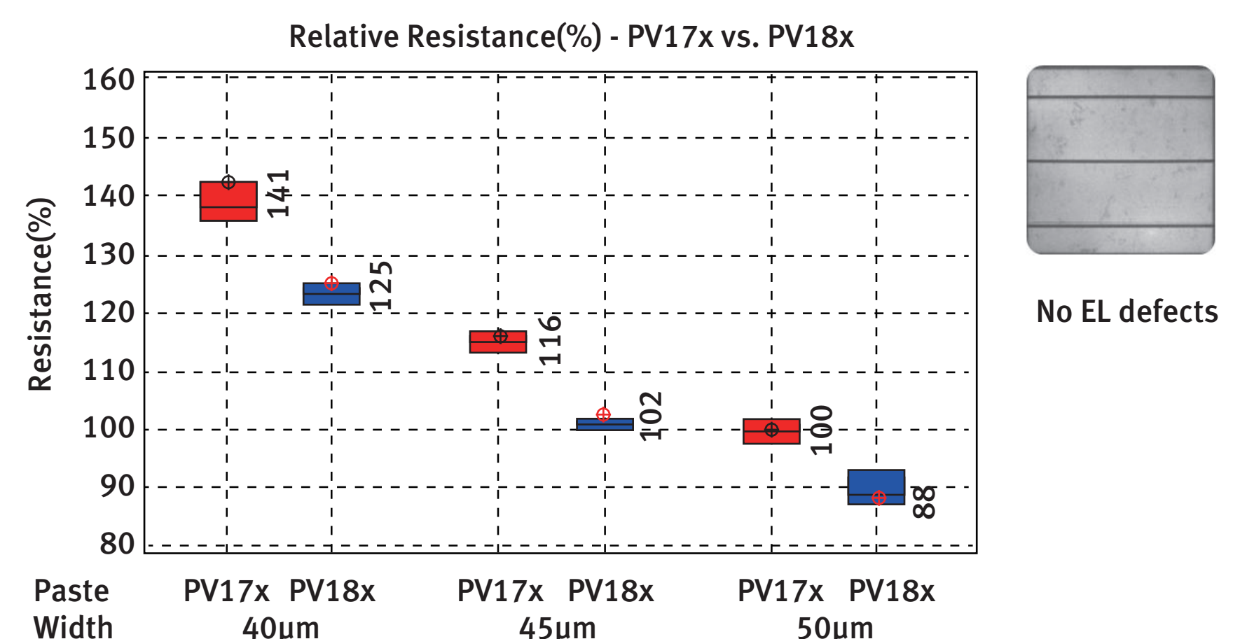
DuPont™ Solamet® PV18x lower R_{gl} by 12% and no EL defects at 40µm finger line opening
