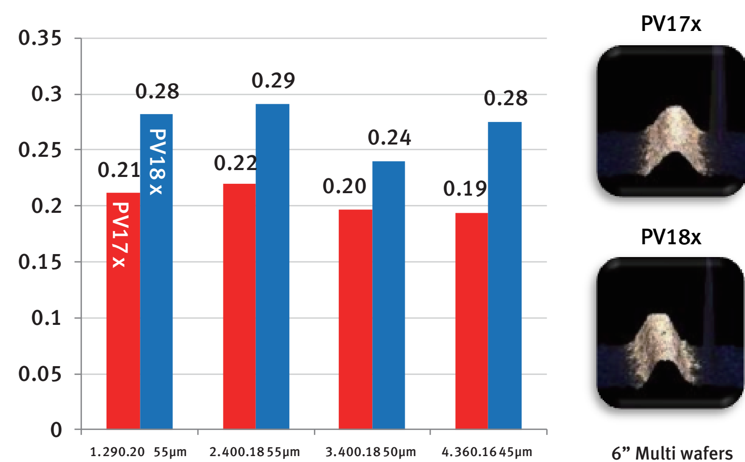
DuPont™ Solamet® PV18x improve aspect ratio with narrow finger line design
